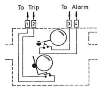
Wiring Diagram Contact position when the relay is oil filled
