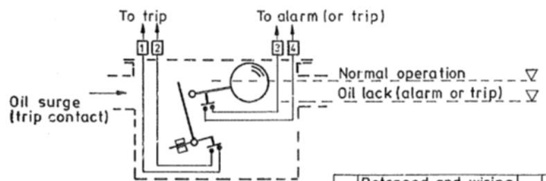
Wiring Diagram
