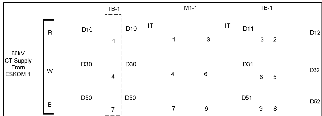
CT Supply from 66kV ESKOM 1
